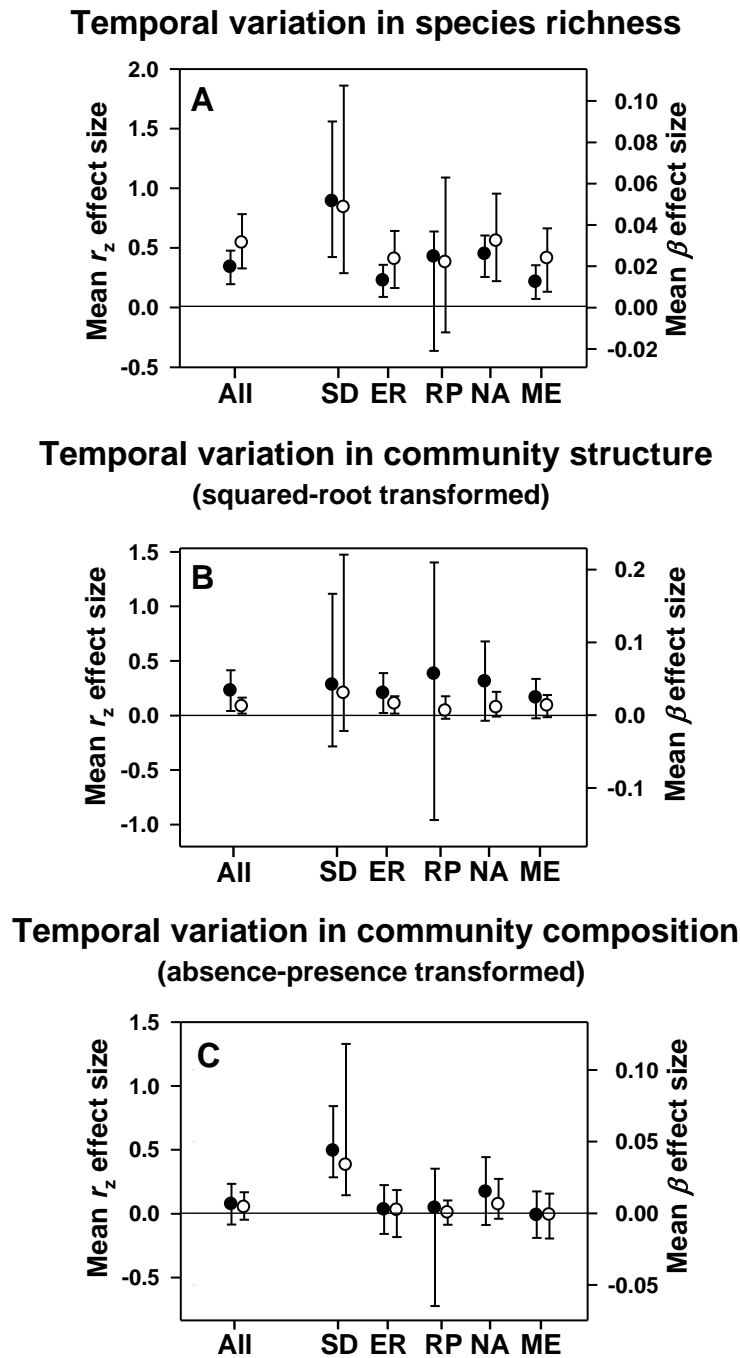
Figure A1. Mean effect size ( \pm 95% CI) for overall effect, by habitat, and by region of the relationship strength r_z (black circle) and slope \beta (open circle) between temporal variability and expected richness E(S_n) at the scale of site. Effect sizes are displayed by type of analysis (species richness variability: A; community assemblage variability in: structure: B; and composition: C). See Figure 2 for abbreviations.
