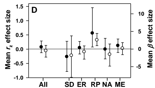
780 Figure 4. Mean effect size ( \pm 95% CI) for overall effect, by habitat, and by region of the relationship strength r_z (black circle) and slope \beta (open circle) between temporal variability in total abundance (density or % cover) and: species richness (A, B), and evenness J' (C, D). Effect sizes are displayed by scale of diversity measure (average by patch scale as quadrat: A, C; reassessed at site scale: B, D). See Figure 2 for abbreviations.
