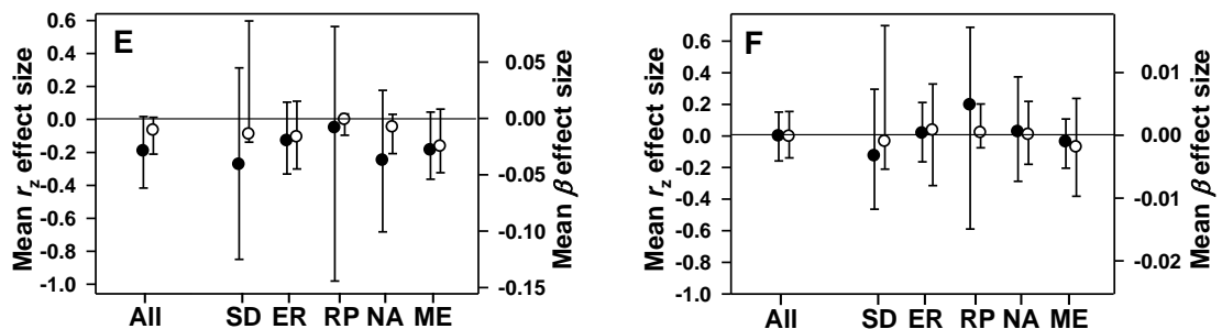
Figure 2. Mean effect size ( \pm 95% CI) for overall effect (All data: All), by habitat (Sediment: SD; Emergent rock: ER; Rock pool: RP), and by region (North Atlantic: NA; Mediterranean: ME) of the relationship strength r_z (black circle) and slope \beta (open circle) between temporal variability and species richness. Effect sizes are displayed by type of analyses (species richness variability: A, B; community assemblage variability in: structure C, D and composition E, F) and scale of richness measure (average by patch scale as Quadrat: A, C, E; total by shore as Site: B, D, F). Horizontal brackets with * indicate significant ( P < 0.05 ) heterogeneity of effect sizes among categories. Significant effects where CIs do not overlap with zero line. Note that negative values indicate a positive stability-diversity relationship while positive values do the opposite.
