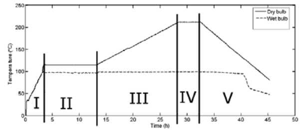
Figure 2 Typical ThermoWood Heat Treatment Schedule (ThermoWood Handbook, 2003)
