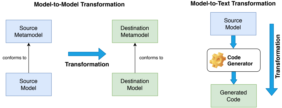
Figure 1.2 : The two types of model transformation
