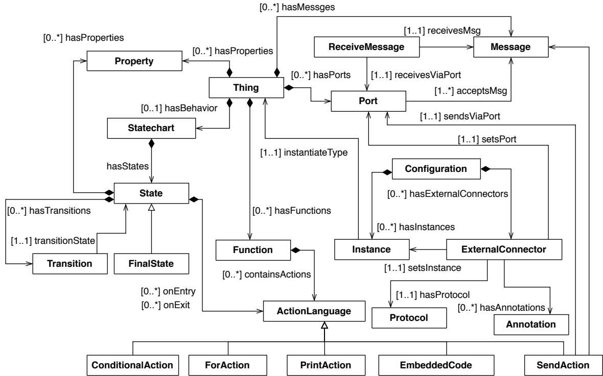
Figure 2.2 : A simplified version of the ThingML metamodel
