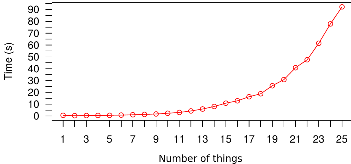
Figure 5.2 : CY-CGEN execution time according to the number of things
