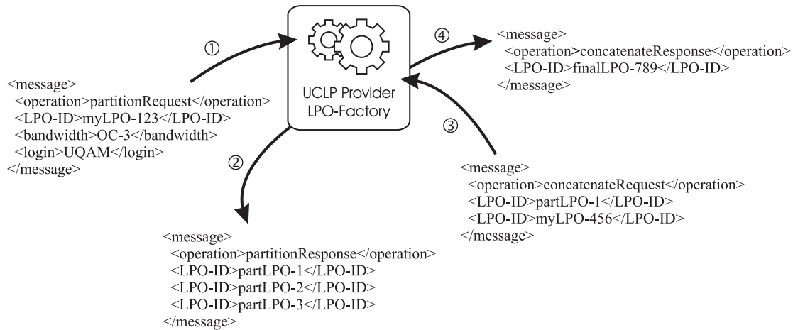
Figure 4. Pattern of messages exchanged between a customer BPEL process and a provider LPO-Factory service
