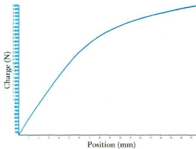
Figure 5.1 : Test de traction.
