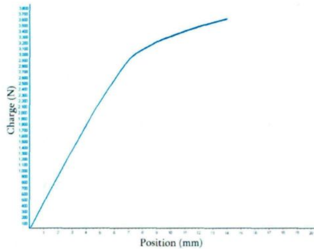
Figure 5.3 : Test de compression.
