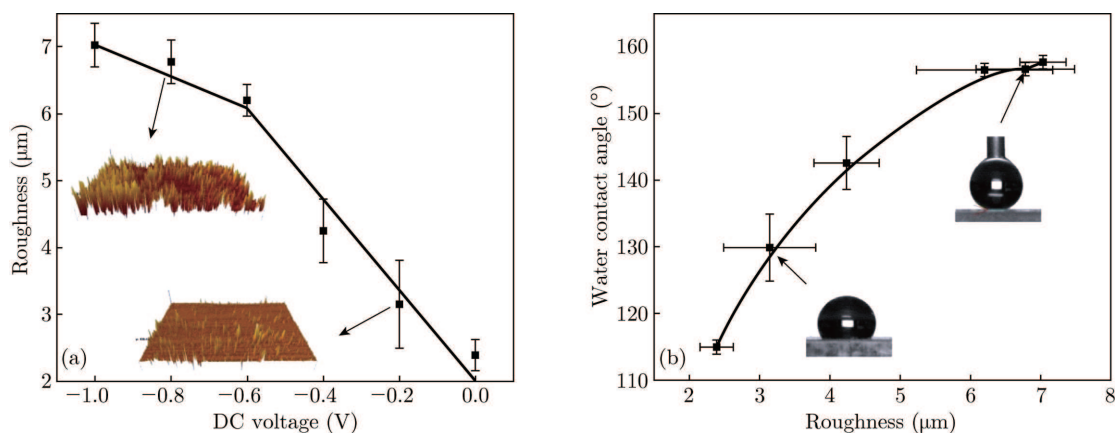
Fig. 4 (a) The variation of roughness vs. deposition potential; (b) variation of water contact angle vs. surface roughness on the stearic acid modified copper film deposited on aluminum surfaces. The inset of (a) shows the 3D images of the rough surfaces and (b) shows the images of water drops ( -0.2 V and -0.8 V).
