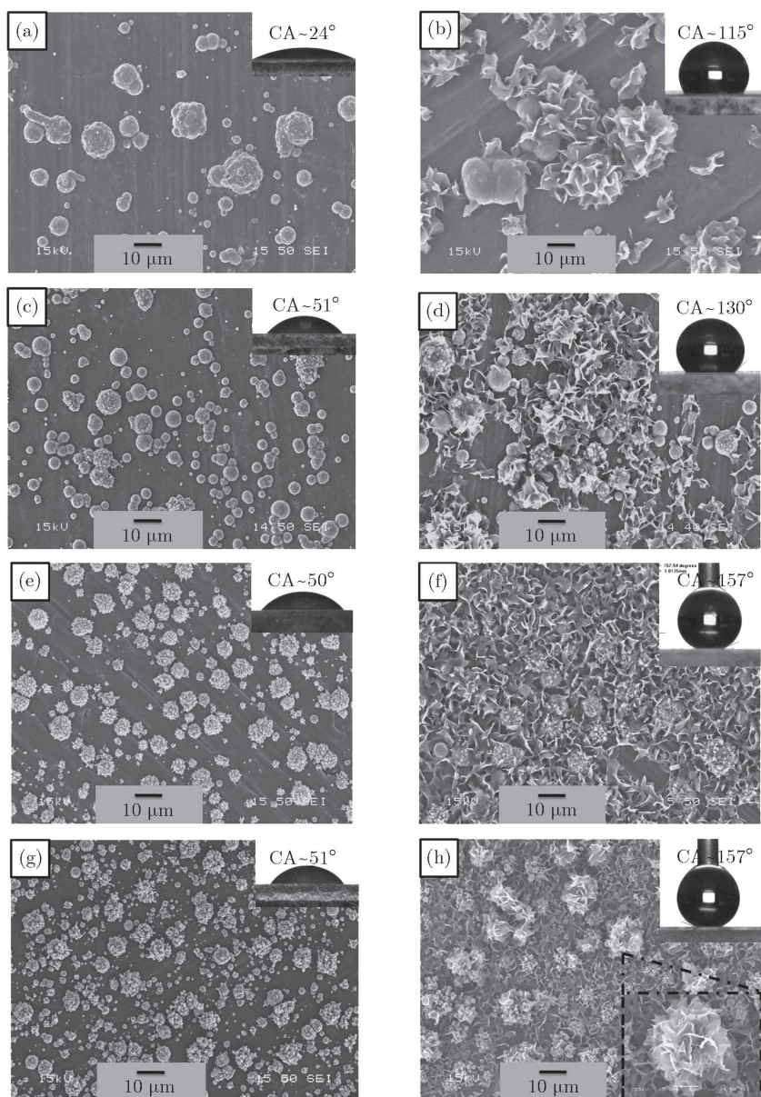
Fig. 1 SEM images (left column) of copper films deposited on aluminum substrates at (a) -0.2 V, (c) -0.4 V, (e) -0.6 V and (g) -0.8 V for 10 minutes. The SEM images (right column) of the same copper films after electrochemical modification in ethanolic stearic acid solution at 30 V for 30 minutes. The insets of Fig. 1 show the images of water drop on the respective surfaces.
