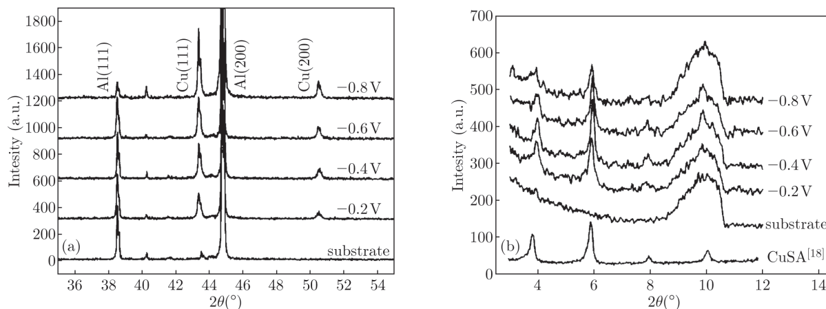
Fig. 3 (a) High angle XRD patterns of copper films deposited on aluminum substrates for the duration of 10 min under the application of various potentials followed by electrochemical modification in ethanolic stearic acid solution; (b) low angle XRD patterns of (a). CuSA is the XRD pattern of copper stearate films as reported by us in [18].
