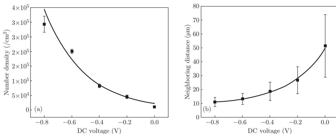
Fig. 2 (a) The number density of the copper microdots as a function of deposition potential, and (b) The distance between the copper microdots as a function of deposition potential.
