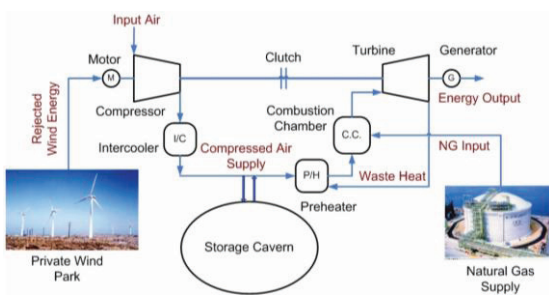
Fig. 5. Wind-Compressed air energy storage hybrid system
