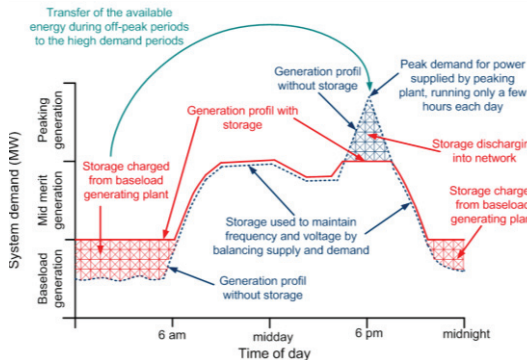
Fig. 3. Fundamental idea of the energy storage [18]
