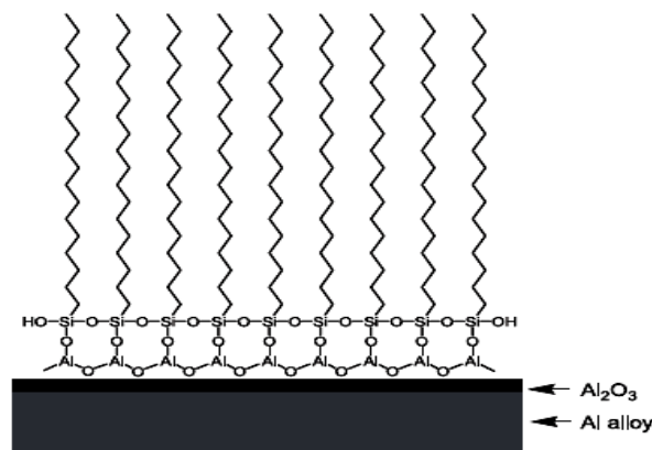
Fig.2.8. Self-assembled monolayer film of alkyldisilane molecules on AA substrate.
