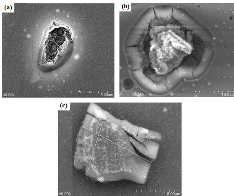
Fig.7.4. SEM images of a) bare Al and coated Al with SAMs of b)18C and c) BTSE/18C coatings after 85 cycles of cyclic corrosion test.
