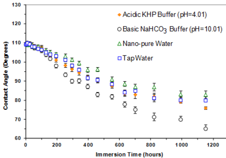
Fig.4.4. Contact angle of Al samples coated with 18C-SAMs vs. immersion time in acidic (pH=4.01), basic (pH=10.01), nano-pure and tap water. At the end of the test, the lowest and highest values of free surface energy ( \epsilon ) are 21.31 ( \pm 0.63 ) and 33.35 ( \pm 0.63 ) mNm^{-1} , respectively.
