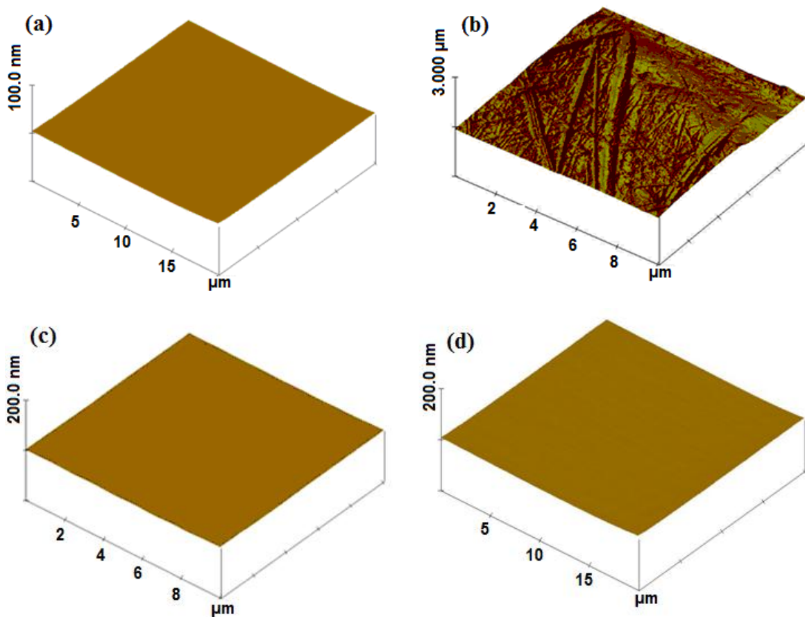
Fig.6.10. AFM images of: (a) bare standard AA2024 ( R_{\text{rms}} : ~ 28 nm), (b) as-received AA2024 ( R_{\text{rms}} : ~ 177 nm) and Al surface coated with (c) single 18C-SAMs ( R_{\text{rms}} : ~ 25 nm) and (d) BTSE/18C-SAMs ( R_{\text{rms}} : ~ 33 nm) prior to test.
