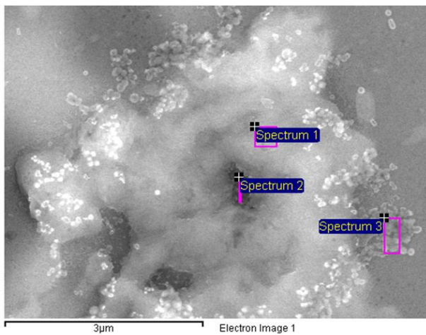
Fig.6.14. EDX results and SEM images of bare standard AA2024 after stability test (immersion in water).
