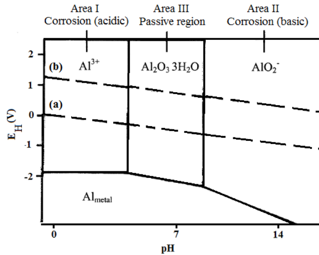
Fig.2.6. Potential vs. pH diagram for Al/H 2 O system at 25 °C and at 1 atm [205].
