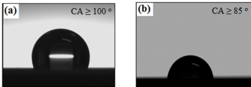
Fig.4.7. Water droplet images on an Al surface coated with 18C-SAMs: a) before [ \epsilon:6.08 (\pm 1.13) \text{ mNm}^{-1} ] and b) after 700-h immersion in nano-pure water [ (\epsilon:21.12 (\pm 1.23) \text{ mNm}^{-1}) ].
