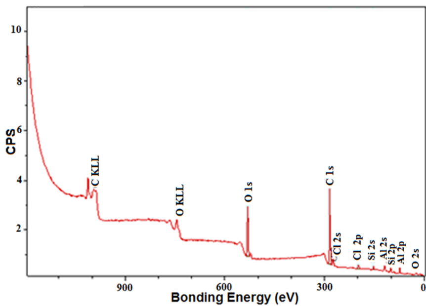
Fig.4.10. XPS spectra of aluminum sample coated with 18C+Cl SAMs coating.
